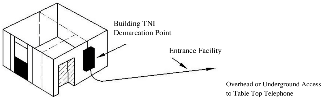
Figure 1: Single small building; one terminal. Impact: Property owner is responsible for inside wire.
